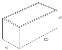
RECTANGULAR PLANTER FIOR200004 ■ 60x120x60 cm
